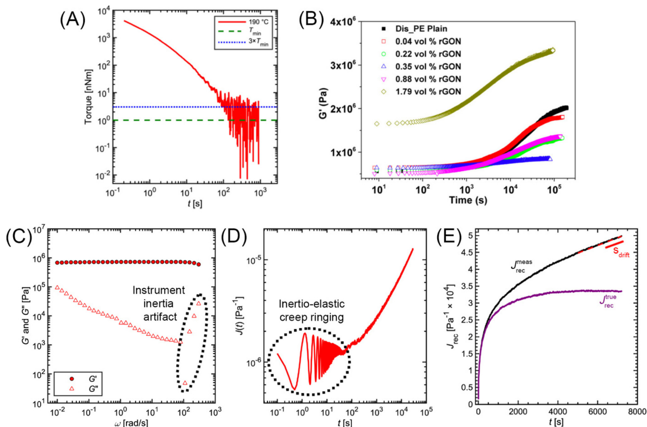
Fig. 14 (A) Minimum torque limits applied to commercial PS stress relaxation data at 190 °C. Data were collected using an Anton Paar MCR 302e rheometer. 3 \times T_{min} was used as the torque cut-off. (B) Time sweep measurements to evaluate thermal degradation of polyethylene containing reduced graphene oxide. Adapted from ref. 73. Copyright 2015 American Chemical Society. (C) G' instrument inertia artifact observed at \omega \geq 100 rad s -1 . (D) Inertio-elastic creep ringing observed in the J(t) of a polybutadiene vitrimer at 160 °C. (C) and (D) Adapted from ref. 92. Copyright 2023 American Chemical Society. (E) Calculation of J_{rec}^{true} for commercial PS at 175 °C.
