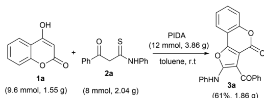
Scheme 2 Gram-scale synthesis of 3a . Reaction conditions: 1a (0.3 mmol), 2a (0.25 mmol), PIDA (12 mmol) and solvent (2.0 mL), room temperature in an open atmosphere.
