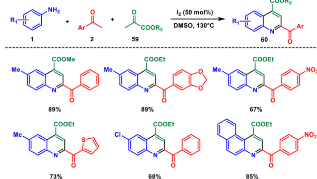
Scheme 24 Iodine-catalysed synthesis through Kornblum oxidation.
