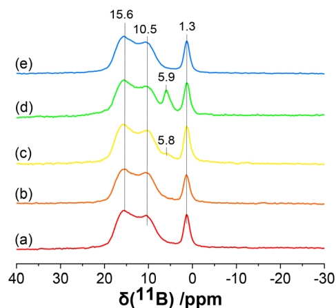
Fig. 3 ^{11}\text{B} MAS NMR of (a) \text{Al}_2\text{O}_3\text{-NaBH}_4(\text{C}) control, (b) \text{Pd}_3/\text{Al}_2\text{O}_3\text{-NaBH}_4(\text{A}) , (c) \text{Pd}_3/\text{Al}_2\text{O}_3\text{-NaBH}_4(\text{B}) , (d) \text{Pd}_3/\text{Al}_2\text{O}_3\text{-NaBH}_4(\text{C}) and (e) \text{Pd}_3/\text{Al}_2\text{O}_3\text{-LiBH}_4(\text{B}) .
