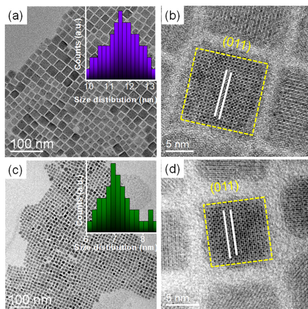
Fig. 1 (a) TEM image of pristine \text{CsPbBr}_3 NCs with an edge dimension of 11.7 \pm 2 \text{ nm} . The inset shows the corresponding size distribution histogram. (b) High-resolution TEM image of pristine \text{CsPbBr}_3 NCs of the (011) plane with a lattice spacing of 0.21 \pm 0.02 \text{ nm} . (c) TEM image of \text{Ni}^{2+} -doped \text{CsPbBr}_3 NCs with an edge dimension of 7.02 \pm 2 \text{ nm} . The inset shows the size distribution histogram. (d) High-resolution TEM image of \text{Ni}^{2+} -doped \text{CsPbBr}_3 NCs showing a lattice spacing of 0.19 \pm 0.02 \text{ nm} for the (011) plane.
