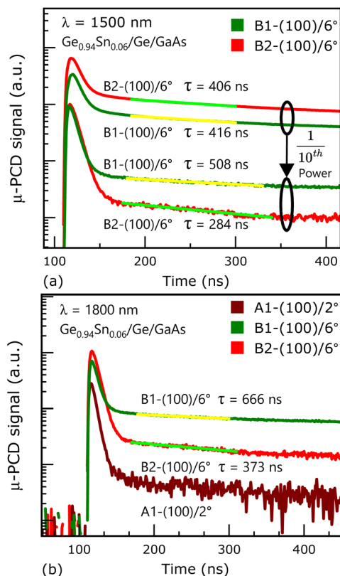
Fig. 9 \mu -PCD measurement data acquired from (100)/6° Ge 0.94 Sn 0.06 samples B1 and B2 at 300 K using: (a) 1500 nm excitation wavelength with an order of difference in excitation power; (b) 1800 nm excitation wavelength, where sample A1 is also shown. The minority carrier lifetimes obtained for sample B1 (100 nm thick epilayer was grown at 185/150 °C) is higher than sample B2 (50 nm thick epilayer was grown at 225 °C) at both excitation wavelengths, due to thickness and growth temperature. 16 It is observed that for sample A1 (100)/2°, the signal is too noisy to extract the lifetime further indicating that (100)/6° orientation offers better quality growth of GeSn epitaxy.
