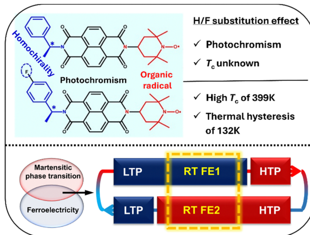
Fig. 14 Effects of H/F substitution in NDI derivatives (top) and the combination of martensitic phase transition and ferroelectricity in S -/ R -F NDI derivatives with two different ferroelectric phases at room temperature (bottom). LTP and HTP represent the low-temperature phase and high-temperature phase, respectively. RT FE1 and RT FE2 represent different ferroelectric phases at room temperature (adapted and modified from ref. 132).
