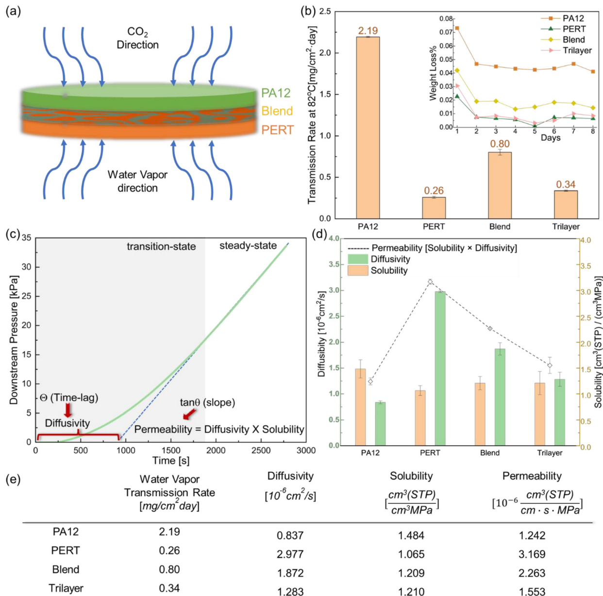
Fig. 3 Barrier properties, i.e. , water vapor and \text{CO}_2 permeability, of PA12, PERT, Blend and Trilayer. (a) Schematics of permeation test on water vapor and \text{CO}_2 with different transmission directions. (b) Measured weight loss % of water vapor and calculated transmission rate at 82 °C. Trilayer sample showed comparable water vapor barrier property to PERT. (c) Example of downstream pressure vs. time curve from \text{CO}_2 permeation test at 82 °C, and extracted \text{CO}_2 permeability from slope, and \text{CO}_2 diffusivity from x-intercept. (d) and (e) Calculated \text{CO}_2 diffusivity, solubility, and permeability of PA12, PERT, Blend, and Trilayer at 82 °C. Trilayer sample showed comparable \text{CO}_2 barrier property to PA12.
