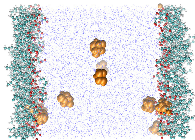
Fig. 7 Snapshot of a typical configuration of a system formed by two interfaces each saturated with 40 nonanoic acid molecules. Ten levoglucosan molecules represented by van der Waals spheres are then added to the system.
