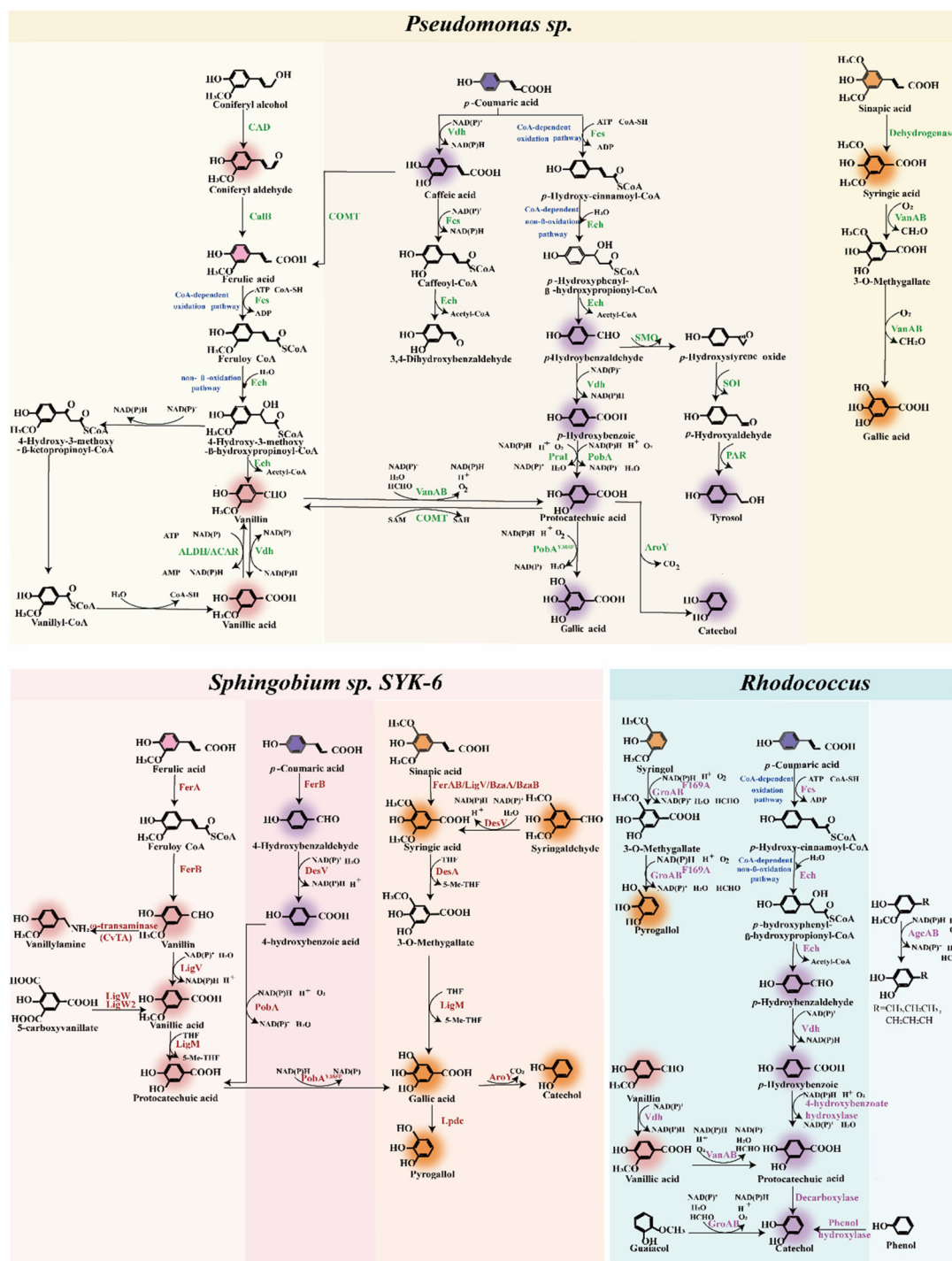
Fig. 3 Inherent lignin biological funneling pathways of representative ligninolytic strains, mainly including Pseudomonas sp. , Sphingobium sp. , and Rhodococcus . Pink color patches represent G-type monomers and related aromatic chemicals. Purple color patches represent H-type monomers and related aromatic chemicals. Orange color patches represent S-type monomers and related aromatic chemicals. ACAR, aromatic carboxylic acid reductase; AgcAB, CYP255A1 family P450; ALDH, acetaldehyde dehydrogenase; AroY, protocatechuate decarboxylase; BzaAB, hydroxybenzimidazole synthase; CAD, coniferyl alcohol dehydrogenase; CalB, lipase B from Candida Antarctica ; COMT, caffeate O-methyltransferase; CvTA, amine transaminases from C. violaceum ; DesV, aromatic aldehyde dehydrogenase; Ech, enoyl-CoA hydratase; Fcs, acyl-CoA synthetase; FerA, feruloyl-CoA synthetase; FerB, feruloyl-CoA hydratase/lyase; GroAB, GcoAB cytochrome P450 system comprises a coupled monooxygenase (GcoA) and reductase (GcoB) that catalyzes oxidative demethylation of the O-methoxy-aryl group in guaiacol; LigM, Vanillate/3-O-methylgallate O-demethylase; LigV, vanillin dehydrogenase; LigW, 5-carboxyvanillate decarboxylase; LpdC, gallate decarboxylase; PAR, phenylacetaldehyde reductase from Solanum lycopersicum ; PobaA, p -hydroxybenzoate hydroxylase; Poba**, the mutant of p -hydroxybenzoate hydroxylase; Poba Y385F , a mutant of a para -hydroxybenzoic acid hydroxylase with improved substrate specificity for PCA; Pral, p -hydroxybenzoate hydroxylase; SMO, styrene monooxygenase; SOI, styrene oxide isomerase; VanAB, vanillate O-demethylase oxygenase; Vdh, vanillin dehydrogenase.
