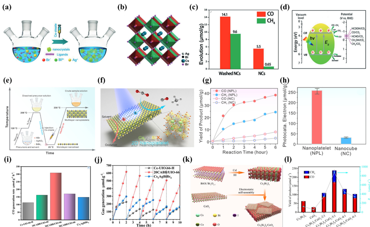
Fig. 6 (a) Schematic illustration of the solution phase synthesis of \text{Cs}_2\text{AgBiBr}_6 NPs (hot-injection route). 84 (b) Crystal structure of cubic \text{Cs}_2\text{AgBiBr}_6 . 84 (c) Comparison of the photocatalytic \text{CO}_2 reduction performance of the as-prepared \text{Cs}_2\text{AgBiBr}_6 NPs and washed NPs. 84 (d) Schematic diagram of the photocatalytic \text{CO}_2 reduction on the surface of \text{Cs}_2\text{AgBiBr}_6 NPs. 84 (e) Schematic illustration of the synthetic procedure of lead-free \text{Cs}_2\text{AgBiBr}_6 double perovskite 2D NPLs. 85 (f) Schematic illustration of the \text{Cs}_2\text{AgBiBr}_6 NPL photocatalyzed \text{CO}_2 reduction reaction. 85 (g) CO (red) and \text{CH}_4 (blue) product yield evolution as a function of reaction time using \text{Cs}_2\text{AgBiBr}_6 double perovskite NPLs (solid) and NPs (open) as catalysts. 85 (h) Histogram of the total photocatalytic electron consumption in 6 h for the reactions using \text{Cs}_2\text{AgBiBr}_6 double perovskite NPLs (red) and NPs (blue) as catalysts. 85 (i) CO generation rate during \text{CO}_2 reduction under 300 W Xe lamp irradiation with as-prepared samples. 45 (j) The recycling test for the photocatalytic activity of \text{Ce-Uio-66-H} , 20\text{CABB}/\text{Uio-66} , and \text{Cs}_2\text{AgBiBr}_6 . 45 (k) The preparation of \text{Cs}_3\text{Bi}_2\text{I}_9 nanosheets and the self-assembly between \text{Cs}_3\text{Bi}_2\text{I}_9 and \text{CeO}_2 nanosheets. 86 (l) The yields of CO and \text{CH}_4 over \text{Cs}_3\text{Bi}_2\text{I}_9 , \text{CeO}_2 and \text{Cs}_3\text{Bi}_2\text{I}_9/\text{CeO}_2 -x:1 (x = 2–6) in 12 h. 86
