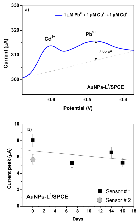
Fig. 12 (a) Selectivity test of the various HMI ions ( Pb^{2+} , Cu^{2+} , and Cd^{2+} ) at 1 \mu M in seawater and (b) reproducibility test of two AuNPs-L 1 /SPCE sensors and signal stability test up to 16 days.
