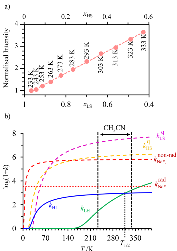
Fig. 10 (a) Steady-state Nd( ^4F_{3/2} ) NIR luminescence monitoring of the Fe(II) spin-state in the dinuclear [\text{Fe(II)Nd(L10)}_3]^{5+} helicite in acetonitrile ( x_{\text{LS}} = 1 - x_{\text{HS}} is the mole fraction of low-spin Fe(II)) and (b) associated kinetic rate constants (see Fig. 8 for the kinetic scheme). This figure has been adapted from ref. 77 with permission from American Chemical Society, copyright 2024.
