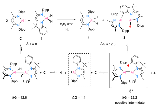
Scheme 4 Possible dialumene intermediate 3* for the reaction of 1 with excess [\text{DippBDIAL}] ( C ). Intramolecular C–H activation forms compound 3 at 85^\circ\text{C} after 1 day. Free energies ( \Delta G ), given in \text{kcal mol}^{-1} , are relative to the initial reactants, [\text{DippBDIAL}] + [\text{DNIAlH}_2] ( C + 1 ).
