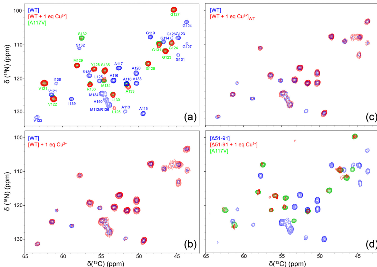
Fig. 3 2D ^{15}\text{N} – ^{13}\text{C}\alpha solid-state NMR chemical shift correlation spectra (red contours) of amyloid fibrils formed by (a) WT huPrP23-144 containing one molar equivalent of bound \text{Cu}^{2+} , (b) WT huPrP23-144 incubated with one molar equivalent of \text{Cu}^{2+} following fibril formation, (c) WT huPrP23-144 containing one molar equivalent of bound \text{Cu}^{2+} seeded with 2% (w/w) pre-formed WT huPrP23-144 fibrils, and (d) \Delta 51 -91 huPrP23-144 containing one molar equivalent of bound \text{Cu}^{2+} . As appropriate, the spectra are overlaid with reference spectra corresponding to WT [panels (a)–(c)] or \Delta 51 -91 huPrP23-144 [panel (d)] fibrils (blue contours) and huPrP23-144 A117V fibrils (green contours) with resonance assignments shown in panel (a). All spectra were recorded at 800 MHz, 11.111 kHz MAS rate and effective sample temperature of ca. 5 °C.
