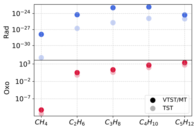
Fig. 3 Rate coefficients ( \text{s}^{-1} ) at 200 K for rad (blue) and oxo (red) mechanisms, demonstrating the contributions of multidimensional tunneling ( \kappa_{\text{SCT}} ) across various substrate chain lengths. The darker circles represent rate coefficients calculated using variational transition state theory with multidimensional tunneling (VTST/MT), while the lighter circles correspond to those obtained from conventional transition state theory (TST) that excludes tunneling contributions.
