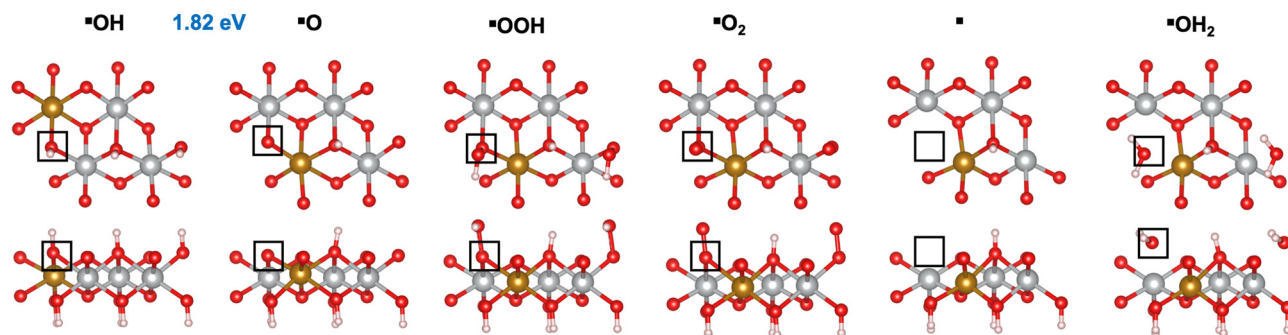
Fig. 3 Atomic structures of the intermediates involved in the OER mechanism with the lowest overpotential on the Fe-doped \bullet OH site ( \blacksquare ) on \beta -NiOOH(0001) relaxed using DFT-HSE06 ( \alpha = 15\% ). The ONIOM Gibbs free energy change corresponding to the PDS is shown in blue. Top panels: Top-down view. Bottom panels: Side view. The empty squares mark the location of oxygen-containing species at the active site. We show only the top layer for clarity. Brown sphere: Fe, grey: Ni, red: O, and pink: H.
