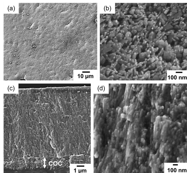
Fig. 5 SEM images (a–d) of the film after overgrowth in aqueous solution with putrescine, [\text{Ca}^{2+}] = 20 \text{ mmol dm}^{-3} , [\text{Mg}^{2+}] = 30 \text{ mmol dm}^{-3} , and [\text{COO}^-_{\text{alginate}}] = 0.5 \text{ mmol dm}^{-3} for 3 h. Top (a and b) and cross-sectional (c and d) views of the film.
