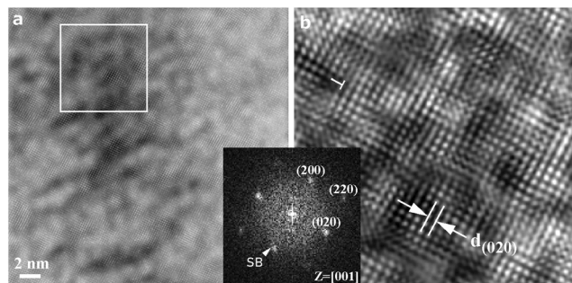
Fig. 5 TEM (a) lattice image of the R-Ti 1-x O rich domain and (b) magnified square region with FFT (inset) showing dislocation (L) and paracrystalline distribution of defect clusters with an interspacing ca. 5 times (020) lattice fringes corresponding to sideband (SB) diffractions in the [001] R zone axis. FIB sample from a film deposited on the FTO-coated silica glass under 200 mJ per pulse.
