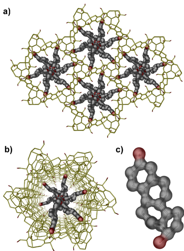
Fig. 3 (a) View along the crystallographic c axis of the porous structure of bioMOF Cu 6 CaSer , prepared from the natural amino acid L-serine, encapsulating the hormone 17-β-estradiol. (b) Perspective view of one single-channel of the hybrid host-guest material. (c) Chemical structure of 17-β-estradiol. The networks are depicted as gold sticks whereas guest molecules are represented as red (oxygen), green (chloride), blue (nitrogen) and gray (carbon) stick/solid surfaces, respectively.
