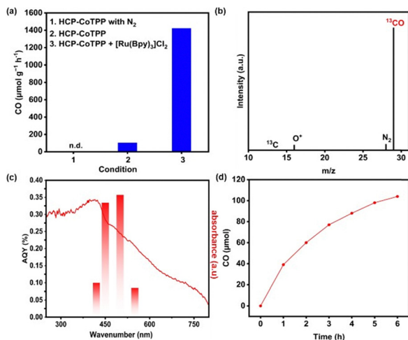
Fig. 3 (a) The photocatalytic \text{CO}_2 conversion rate under different conditions using CoTPP as a catalyst and visible light irradiation ( \lambda \geq 420 nm). Condition 1: under \text{N}_2 , conditions 2 and 3: under \text{CO}_2 , (b) mass spectrum of ^{13}\text{CO} produced using HCP-CoTPP as the catalyst in the photocatalytic reduction of ^{13}\text{CO}_2 , (c) apparent quantum yield (AQY) of \text{CO}_2 photocatalytic reduction for HCP-CoTPP at different wavelengths, (d) CO evolution by HCP-CoTPP (10 mg) with the presence of [\text{Ru}(\text{Bpy})_3]\text{Cl}_2 = (10 mg) within 6 hours.
