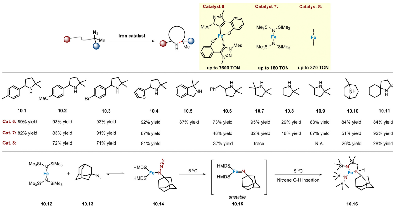
Scheme 10 Mesoiocarbene-iron complex, Fe(HMDS) 2 - and FeI 2 -catalysed intramolecular C(sp 3 )-H amination of alkyl azides.
