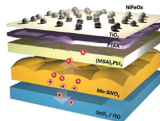
Fig. 40 Pictorial representation, along with the hole transport mechanism, of the oxygen evolution reaction device. Reprinted with permission from ref. 72 Copyright©2023 Wiley-VCH GmbH.
