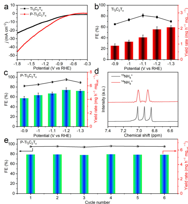
Fig. 2 (a) LSV curves in NO 3 − -containing electrolytes in an H cell. (b) and (c) The obtained FEs and yield rates for Ti 3 C 2 T x and P-Ti 3 C 2 T x . (d) The 15 H NMR spectrum. (e) Cycling stability.
