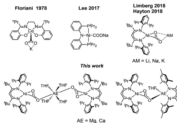
Fig. 1 Selected examples of Alkali metal stabilised \text{CO}_2 complexes.
