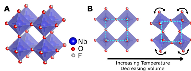
Fig. 1 (A) The cubic ReO 3 -type structure of NbO 2 F in the Pm \bar{3} m space group. (B) An illustration of the rigid unit mode mechanism of negative thermal expansion in the cubic ReO 3 -type structure.
