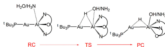
Scheme 10 Sketched structures of the stationary points along the reaction profile calculated for the O–H/N–H bond activation of \text{H}_2\text{O}/\text{NH}_3 with the \text{Au} – \text{Al} bond. RC = reactant complex, TS = transition state, PC = product complex.
