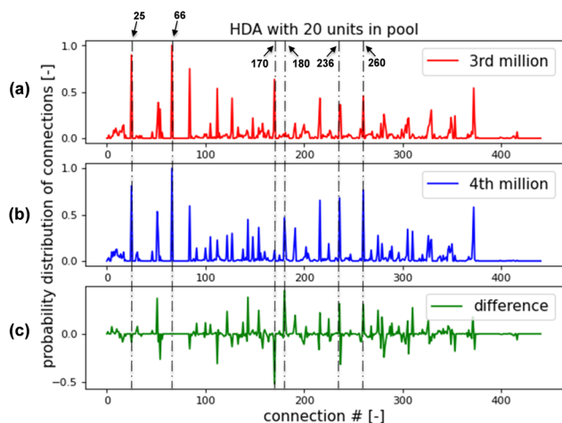
Fig. 16 Probability distribution function of connections for HDA system with 20 units in pool. (a) for feasible flowsheets found within the 3rd million of episodes; (b) for feasible flowsheets found within the 4th million of episodes; (c) Difference between (b) and (a).
