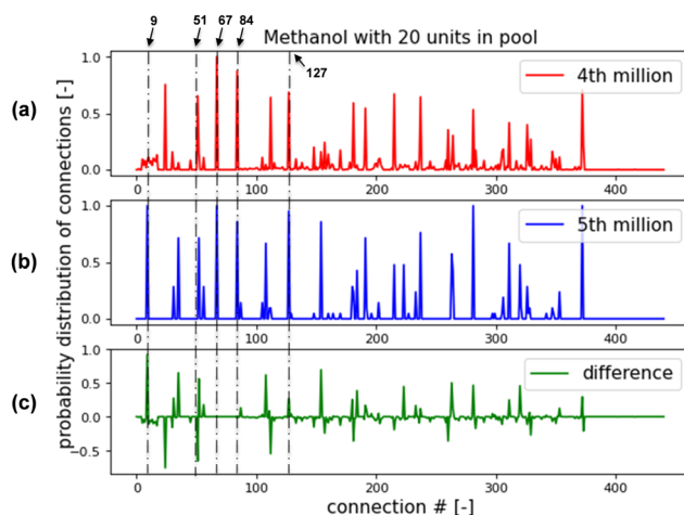
Fig. 17 Probability distribution function of connections for methanol system with 20 units in pool. (a) for feasible flowsheets found within the 4th million of episodes; (b) for feasible flowsheets found within the 5th million of episodes; (c) Difference between (b) and (a).
