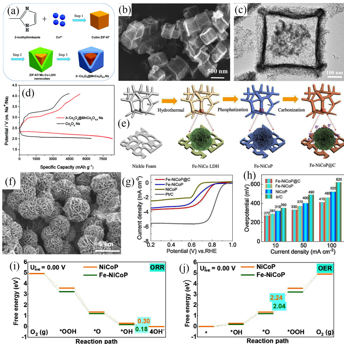
Fig. 17 (a) Scheme for the preparation of h-Co 3 O 4 @MnCo 2 O 4.5 Ns. (b) The SEM image and (c) The TEM image of h-Co 3 O 4 @MnCo 2 O 4.5 Ns. (d) The initial discharge/charge profiles of Na-O 2 batteries with h-Co 3 O 4 @MnCo 2 O 4.5 Ns and Co 3 O 4 Ns electrodes. (Reproduced from ref. 156 with permission from the Royal Society of Chemistry). (e) Scheme for the preparation of Fe-NiCoP@C. (f) The SEM image of Fe-NiCoP@C. (g) ORR polarization curves of NiCoP, Fe-NiCoP, Fe-NiCoP@C, and Pt/C electrode. (h) The overpotentials of NiCoP, Fe-NiCoP, Fe-NiCoP@C, and Ir/C electrode. (i and j) Calculated OER/ORR energy diagram of the NiCoP and Fe-NiCoP. (Reproduced from ref. 17 with permission from the Elsevier).
