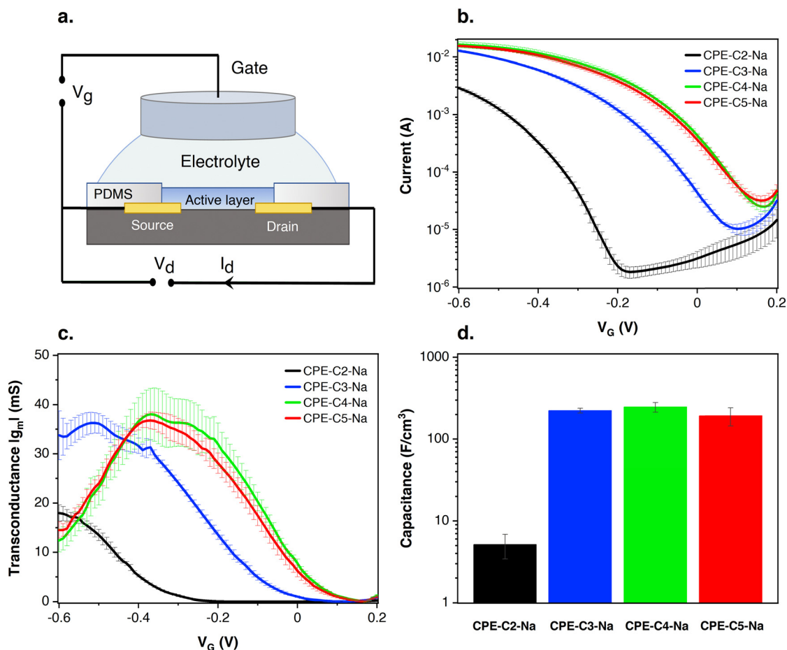
Fig. 7 (a) Device architecture of CPE-based OEETs; (b) transfer characteristics at V_D = -0.6 V of OEETs made using interdigitated contacts ( W = 27 cm, L = 8 \mu m, d = 1.5 – 1.9 \mu m); (c) transconductance values at V_D = -0.6 V of OEETs made with interdigitated contacts. (d) Volumetric capacitance measured by impedance spectroscopy.
