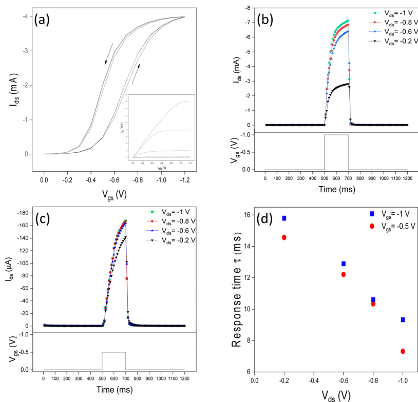
Fig. 2 Characteristics of [EMIM][TFSI]-gated P3HT transistors. (a) Transfer characteristics in the linear regime ( V_{ds} = -0.2 V, (3 cycles) at V_{gs} 100 \text{ mV s}^{-1} scan rate (inset: output characteristic with V_{gs} = 0, -0.2, -0.4, -0.6, -0.8, -1 V and V_{ds} 100 \text{ mV s}^{-1} scan rate). I_{ds} response to (b) V_{gs} = -1 V, (c) V_{gs} = -0.5 V, at different V_{ds} . The duration time of the V_{gs} bias is 200 ms. (d) Transient response of an [EMIM][TFSI]-gated P3HT transistor versus V_{ds} in different values of V_{gs} square step.
