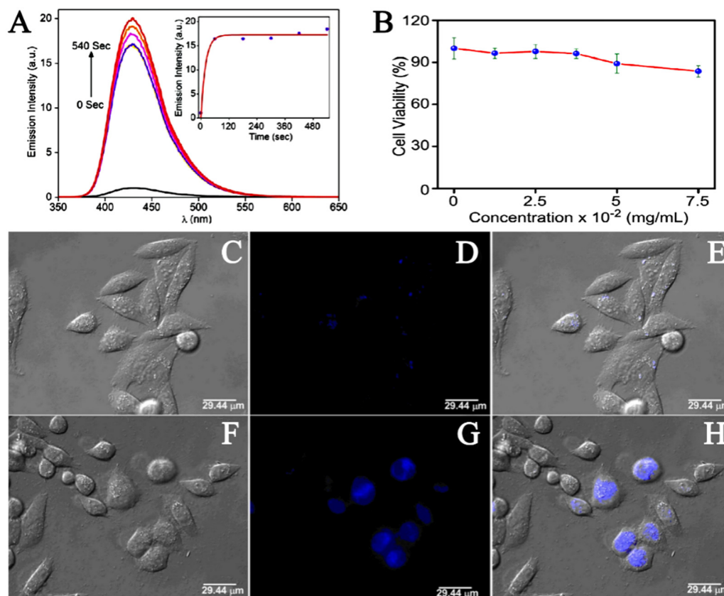
Fig. 10 (A) Fluorescence response of 1- \text{N}_3 towards the addition of \text{Na}_2\text{S} after 0, 60, 180, 300, 420 and 540 seconds. Inset: Time dependence of emission intensity at 436 nm. (B) HeLa cells were treated with 1- \text{N}_3 before adding MTT for 6 h. Results are expressed as % of the control (100%). (C–E) Fluorescence imaging of HeLa cells incubated with 1- \text{N}_3 . (F–H) Fluorescence imaging of HeLa cells incubated with \text{Na}_2\text{S} . 80 Reproduced with permission. Copyright 2014, Springer Nature.
