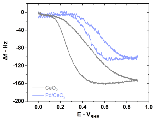
Fig. 7 EQCM measurements on pure CeO 2 reveals the role played by the support on Pd/CeO 2 represented by the difference in frequency during HOR. Reaction conditions: 5 \text{mV s}^{-1} scan rate, H 2 -saturated 0.1 M KOH solution.
