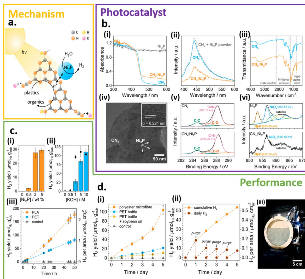
Fig. 7 (a) Schematic diagram of the polymer photoreforming process using \text{CN}_x|\text{Ni}_2\text{P} photocatalyst. (b) Characterization of the \text{CN}_x|\text{Ni}_2\text{P} (2 wt%) photocatalyst. Comparison of (i) diffuse-reflectance UV-vis, (ii) emission ( \lambda_{\text{ex}} = 360 \text{ nm} , \lambda_{\text{em}} = 450 \text{ nm} ), and (iii) FTIR spectra of \text{CN}_x and \text{CN}_x|\text{Ni}_2\text{P} . (iv) TEM image of the \text{CN}_x|\text{Ni}_2\text{P} catalyst, with the inset showing the lattice spacing of \text{Ni}_2\text{P} . XPS spectra of (v) \text{C}_{1s} edge for \text{CN}_x and \text{CN}_x|\text{Ni}_2\text{P} and (vi) \text{Ni}_{2p} edge for \text{Ni}_2\text{P} and \text{CN}_x|\text{Ni}_2\text{P} . (c) Photoreforming of PET and PLA with \text{CN}_x|\text{Ni}_2\text{P} . Optimization of (i) \text{Ni}_2\text{P} loading and (ii) KOH concentration for the photoreforming of PET (after 20 h irradiation). Black circles in (ii) mark \text{H}_2 evolution per gram of substrate over \text{CN}_x|\text{Pt} (2 wt%) under the same conditions. (iii) Long-term photoreforming of PET and PLA. Conditions unless stated otherwise: \text{CN}_x|\text{Ni}_2\text{P} 2 wt% ( 1.6 \text{ mg mL}^{-1} ), pretreated PET ( 25 \text{ mg mL}^{-1} ), aqueous KOH (1 M, 2 mL), and simulated solar light (AM 1.5 G, 100 \text{ mW cm}^{-2} , 25^\circ \text{C} ). (d) Photoreforming of nonrecyclable plastic waste. (i) Long-term photoreforming of polyester microfibers, a PET bottle, and an oil-coated PET bottle. (ii) Upscaled photoreforming of polyester microfibers, where sample was purged every 24 h. Conditions: \text{CN}_x|\text{Ni}_2\text{P} ( 1.6 \text{ mg mL}^{-1} ), 1 M KOH (2 mL for part (i) and 120 mL for part (ii)), pretreated microfibers ( 5 \text{ mg mL}^{-1} ) or PET bottle ( 25 \text{ mg mL}^{-1} ) without or with soybean oil ( 5 \text{ mg mL}^{-1} ), simulated solar light (AM 1.5 G, 100 \text{ mW cm}^{-2} ). (iii) Photograph of the batch reactor in use. Reproduced with permission from ref. 100. Copyright 2019, the American Chemical Society.
