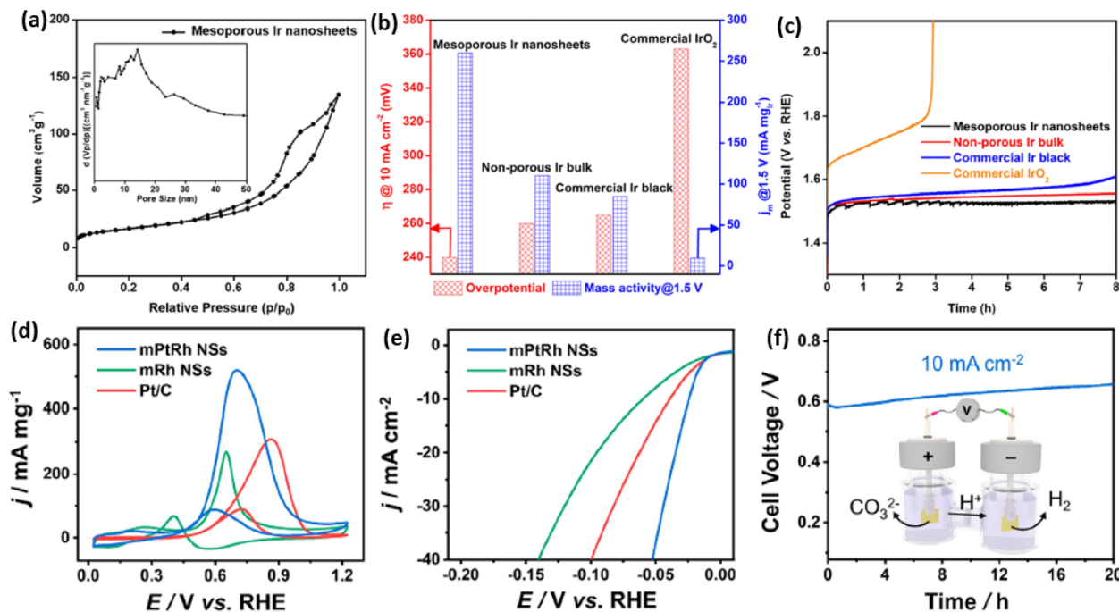
Fig. 6 Enhanced catalytic activity and stability. (a) \text{N}_2 adsorption–desorption isotherm plots of mesoporous Ir nanosheets. (b) Summarized overpotentials (at 10 \text{ mA cm}^{-2} ) and mass activities (at 1.5 \text{ V} ) and (c) chronopotentiometry stability of mesoporous Ir nanosheets and the counterpart electrocatalysts for OER electrocatalysis. Reproduced from ref. 50 with permission from the American Chemical Society, Copyright 2018. (d) CV curves and (e) LSV curves of mesoporous PtRh nanosheets, mesoporous Rh nanosheets, and commercial Pt/C collected in 1.0 \text{ M} KOH methanol solution. (f) Long-term chronoamperometry stability of mesoporous PtRh nanosheets collected in 1.0 \text{ M} KOH methanol solution. Inset in (f) is a schematic illustration of the methanol-assisted \text{H}_2 production process. Reproduced from ref. 64 with permission from the American Chemical Society, Copyright 2022.
