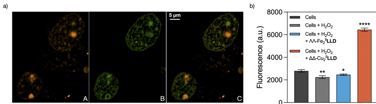
Fig. 6 (a) \Delta\Delta -Cu II 2 TAMRA-L 2 L 2 selectively stains DNA replication sites at the cell nuclei. Vero cells expressing protein GFP-PCNAL2 were incubated in the presence of 25 μg mL -1 of digitonin for 3 min and then in the presence of 5 μM of \Delta\Delta -Cu II 2 TAMRA-L 2 L 2 for 15 min. The Cu II peptide helicate used in these studies was previously assembled before the internalization experiment by adding 5 eq. of CuCl 2 ·2H 2 O to an aqueous solution of TAMRA-L 2 L 2 peptide ligand. (A) Red channel emission showing the distribution of the TAMRA-labelled helicate; (B) green channel, corresponding to the emission of the GFP-PCNAL2 probe that labels DNA replication foci; (C) overlay of the green and red channels, which shows that \Delta\Delta -Cu II 2 TAMRA-L 2 L 2 has localised at the replication foci. Nucleoli are clearly labelled as red spots inside the cell nuclei. The images show a representative confocal section of the Vero cells. (b) Detection of free DNA ends by TUNEL assay. S-phase synchronized Vero cells were incubated with H 2 O 2 alone and with \Lambda\Lambda -Fe II 2 L 2 L 2 or \Delta\Delta -Cu II 2 L 2 L 2 plus H 2 O 2 at 37 °C for 2 hours and then subjected to TUNEL analysis for the detection of free DNA ends. Results are represented as the mean with standard deviation of a triplicate experiment * = P \leq 0.05 ** = P \leq 0.01 *** = P \leq 0.001 and **** = P \leq 0.0001 .
