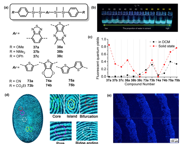
Fig. 9 (a) Chemical structures of DAD and ADA aryldisilanes. (b) Photographs of the photoluminescence of 38a in various THF/water mixtures under 365 nm UV irradiation. Reproduced with permission from ref. 85, Copyright 2016, Wiley-VCH. (c) The absolute fluorescence quantum yields of compounds 37–38 and 73–75 in DCM solution and the solid state. The data in the figure are from ref. 85. (d) High-resolution photographic images of a LFP after treatment with 14 solution, showing level 1–3 details when excited with a 365 nm UV lamp. (e) False-color fluorescence image of the developed LFP showing adhesion of 14 aggregates to ridges. Reproduced with permission from ref. 26, Copyright 2020, Chinese Chemical Society.
