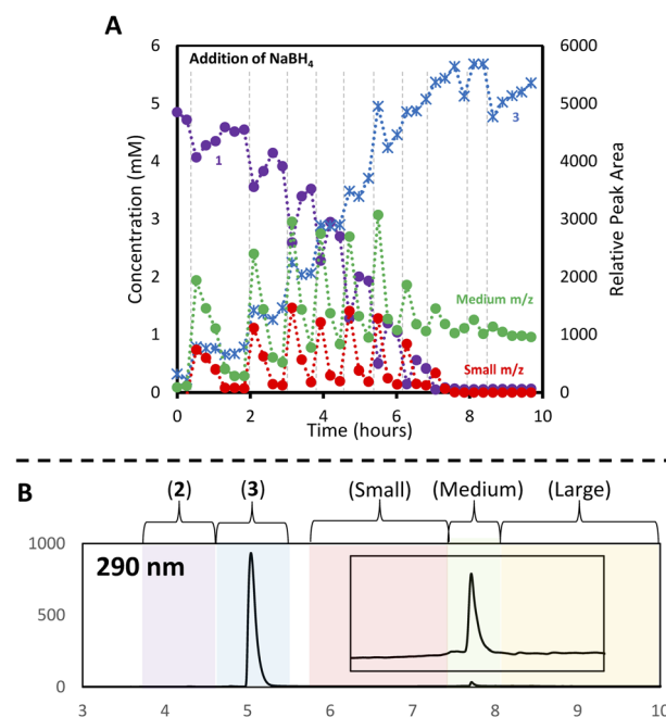
Fig. 10 HPLC time-course for dose-wise synthesis of AuNC 4 . (A) Change in components visualized via regional analysis. Left axis: starting material ( 1 ) and intermediate ( 3 ) quantified via internal standard; right axis: relative integral of respective size region normalized vs. internal standard; red circles (small region), green circles (medium region). Ten equal doses of 0.1 equiv. \text{NaBH}_4 in EtOH added at demarcated times; (B) chromatogram at endpoint reveals 4 is the only persistent AuNC under these conditions.
