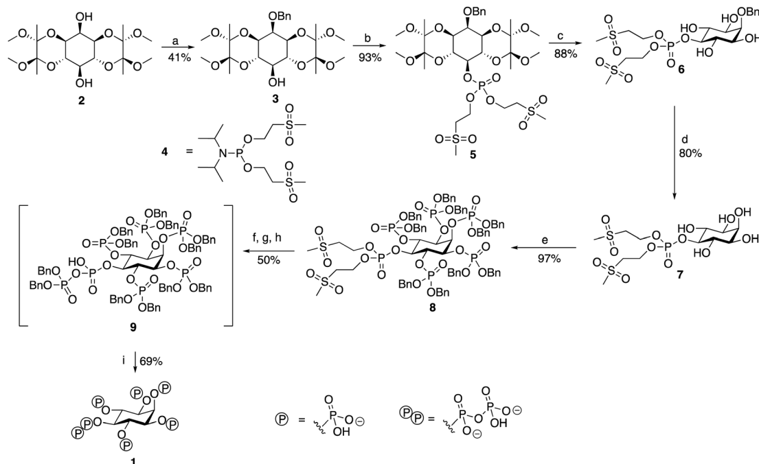
Scheme 1 Synthesis of 5-PP-InsP 5 . Reagents and conditions: (a) DMF, NaH, BnBr; (b) (1) DCM, 5-phenyl-1H-tetrazole, (OMSE) 2 PN(Pr) 2 reagent 4, 16 h (2) m CPBA, −78 °C–RT; (c) TFA, H 2 O; (d) THF, CH 3 COOH, H 2 O, H 2 , Pd(OH) 2 /C; (e) (1) DCM, 5-phenyl-1H-tetrazole, (OBn) 2 PN(Pr) 2 , 16 h (2) m CPBA, −78 °C–RT; (f) DBU, BSTFA; (g) MeOH, TFA; (h) (1) CDCl 3 , 5-phenyl-1H-tetrazole, (OBn) 2 PN(Pr) 2 , 3 h (2) m CPBA, −78 °C–RT; (i) MeOH, THF, 1 M TEAB, H 2 , Pd(OH) 2 /C, 72 h.
