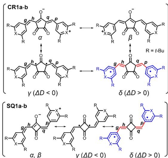
Fig. 6 Resonance structures of CR1a–b and SQ1a–b. Red-highlighted parts indicate methine parts (bonds g, h, p , and q ) with bond length alternation. Blue-highlighted parts are chalcogenopyrylium rings in which unpaired electrons are delocalized. The difference between bond lengths at methine parts \Delta D is obtained as follows; \Delta D = (\text{averaged length of } g, p) - (\text{averaged length of } h, q) .
