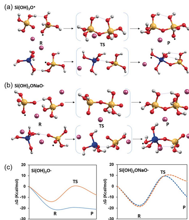
Fig. 3 Optimized geometries of the structures involved in the condensation of (a) \text{Si}(\text{OH})_3\text{O}^\cdot and (b) \text{Si}(\text{OH})_2\text{ONaO}^\cdot radical species with \text{Si}(\text{OH})_3\text{ONa} and \text{Al}(\text{OH})_4\text{Na} . Si, Al, O, H, and Na atoms are depicted as yellow, blue, red, white and purple spheres, respectively. (c) Corresponding Gibbs free energy profiles for condensation of radicals with \text{Si}(\text{OH})_3\text{ONa} (blue) and \text{Al}(\text{OH})_4\text{Na} (orange). Reproduced from ref. 50 with permission from Wiley, Copyright 2020.
