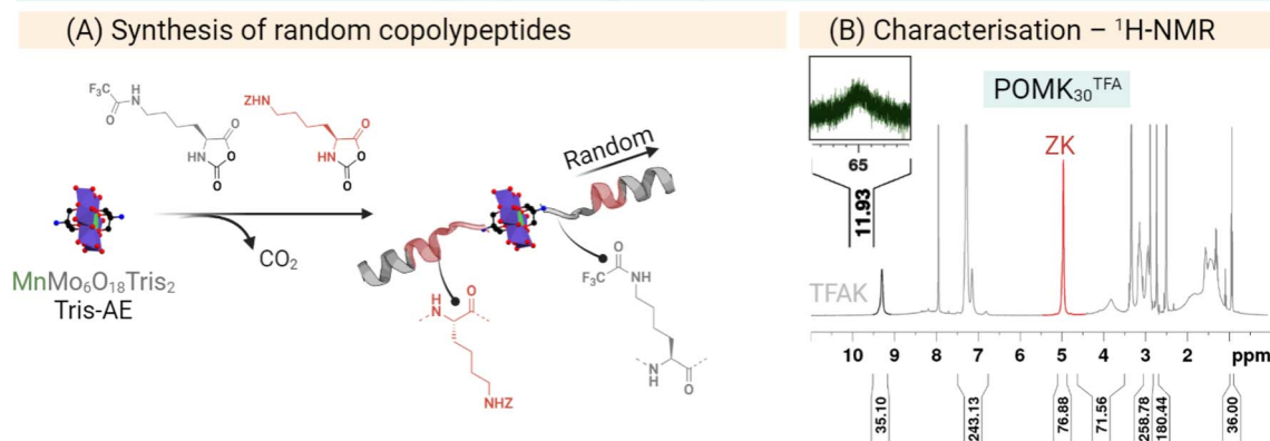
Fig. 10 (A) General scheme for the synthesis of POM polymers from random copolypeptides by the on-POM ring opening polymerisation (ROP) of NCAs – lysine trifluoroacetate NCA (grey, TFA K) and benzyloxycarbonyl lysine NCA (ZK NCA). (B) ^1H -NMR characterisation of POMK_{30}^{TFA} which stands for 30 TFAK residues.
