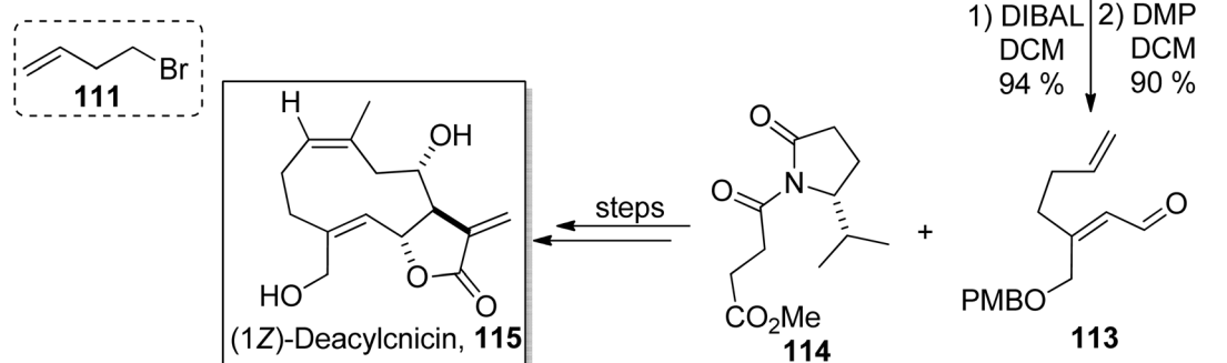
Scheme 12 Total synthesis of (1Z)-deacylnicin 115.
