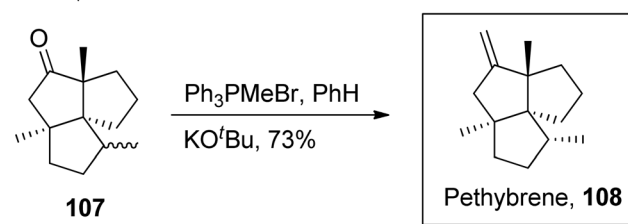
Scheme 11 Total synthesis of pethybrene 108.
