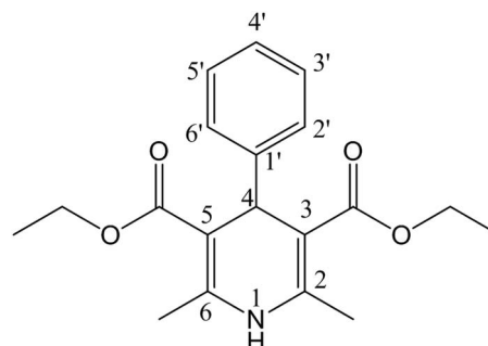
Fig. 1 The 1,4-dihydropyridine [1,4-DHP] moiety.
