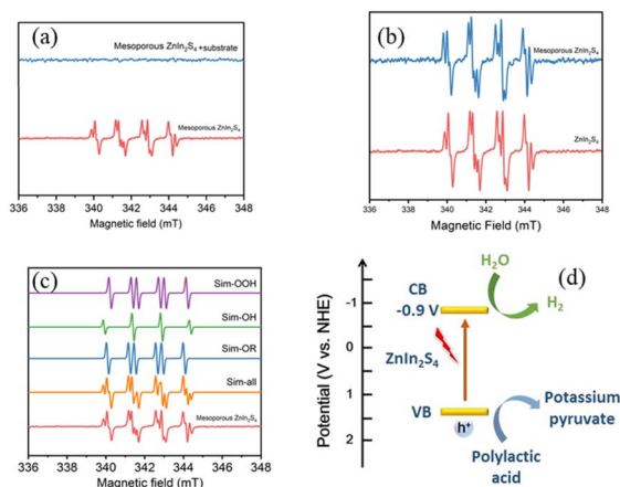
Fig. 8 EPR spectra of free radicals captured by DMPO of (a) mesoporous ZnIn 2 S 4 under simulated solar light with or without substrate; (b) mesoporous ZnIn 2 S 4 and ZnIn 2 S 4 under simulated solar light without substrate (c) simulation of EPR spectra of free radicals captured by DMPO of mesoporous ZnIn 2 S 4 ; (d) proposed mechanism for photoreforming of PLA by mesoporous ZnIn 2 S 4 .
