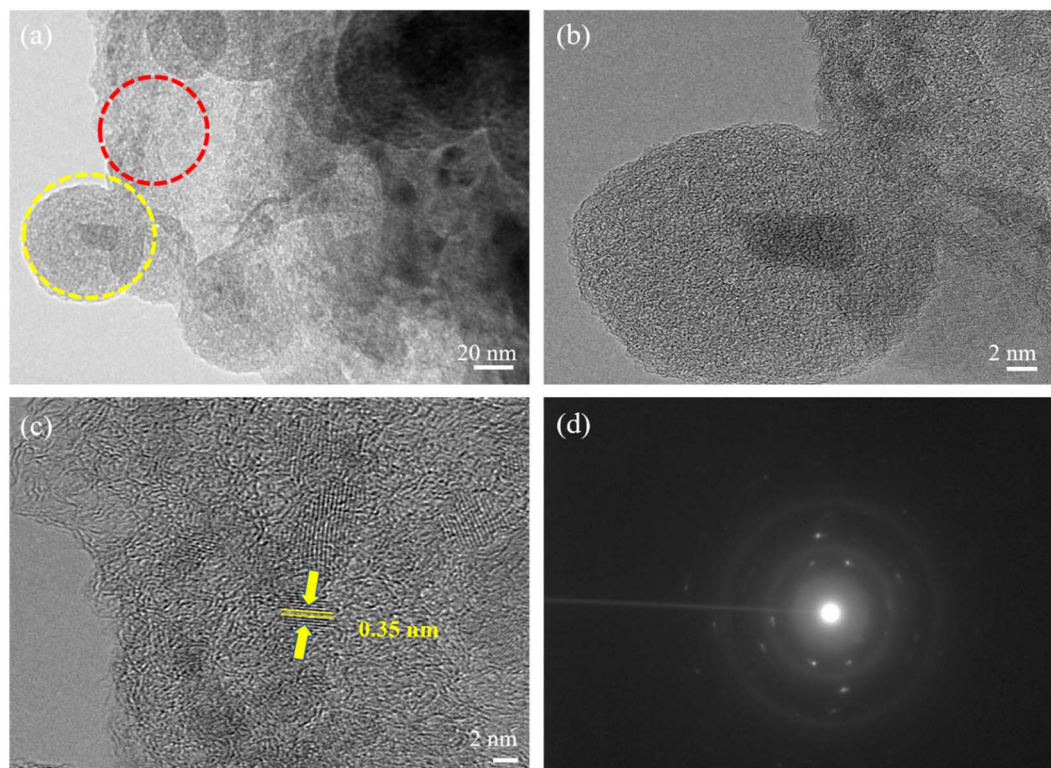
Fig. 3 (a) TEM, (b) HRTEM, [yellow circle area in (a)], and (c) HRTEM [red circle area in (a)] images, and (d) SAED pattern of calcined NMC@MXene-30.
