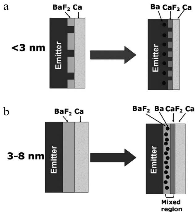
Fig. 7 Schematic diagrams of the contact between the cathode ( \text{BaF}_2/\text{Ca}/\text{Al} ) and the emitter for (a) a thin \text{BaF}_2 layer with a thickness less than 3 \text{ nm} , and (b) a \text{BaF}_2 layer with a thickness of 3-8 \text{ nm} . 155 Copyright 2009 Wiley-VCH Verlag GmbH & Co. KGaA, Weinheim.
