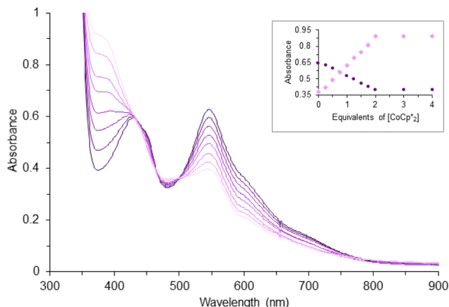
Fig. 3 Reduction of 0.1 mM 1 in THF by addition of CoCp* 2 in increments of 0.25 equiv. as monitored by UV-vis spectroscopy (path length, 1.0 cm). Inset: corresponding changes of the absorbance at 389 (◆) and 545 (●) nm.
