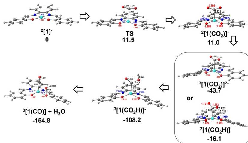
Fig. 10 Optimised structures of the intermediates in CO 2 binding to 2[1]^- and reduction to CO: TS between 2[1]^- and 2[1(CO_2)]^- , 3[1(CO_2)]^{2-} or 2[1(CO_2H)] , 3[1(CO_2H)]^- , and 3[1(CO)] + H_2O .
