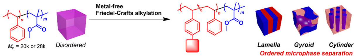
Fig. 1 Chemical modification of PS- b -PMMA. (a) Previous works on the junction point functionalization. (b) Previous works on the PMMA side-chain and chain-end functionalization via post-polymerization modification of commercially available PS- b -PMMA. (c) This work, which focuses on post-polymerization modification of the PS block via the metal-free Friedel-Crafts alkylation reaction.
